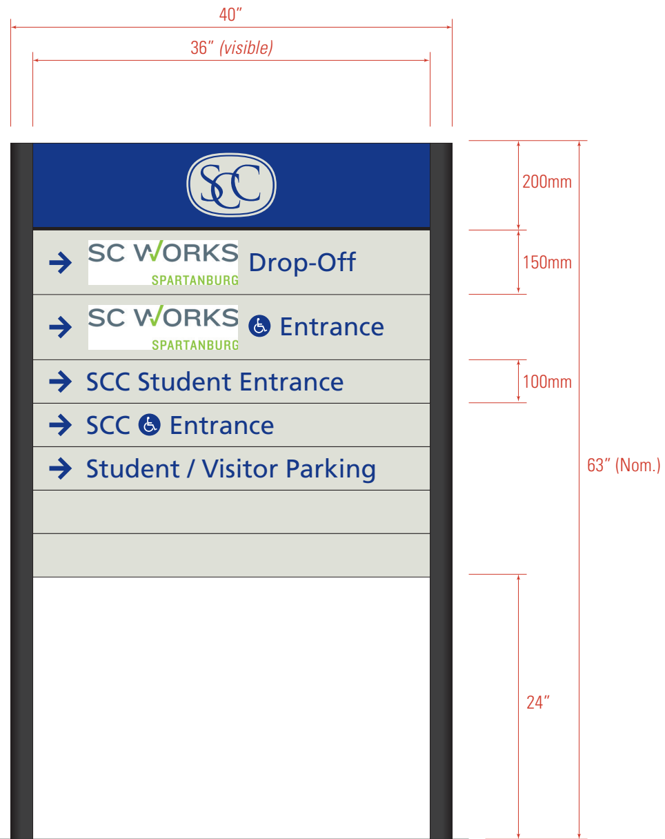
SIDE A - Location: 8 SCALE: 1" = 1'-0"
