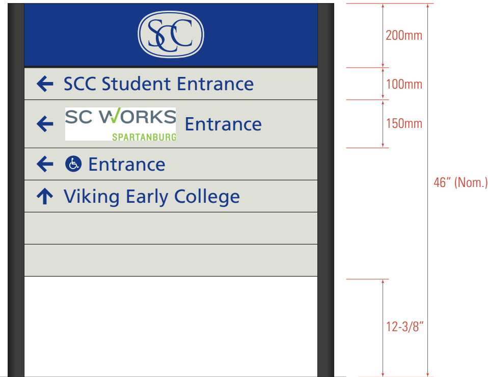
SIDE A - Location: 5 SCALE: 1" = 1'-0"
