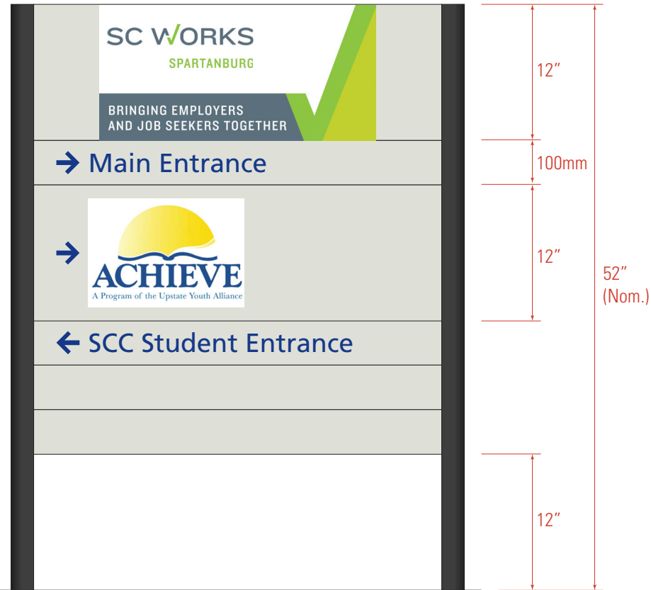
SIDE A - Location: 7 SCALE: 1" = 1'-0"
