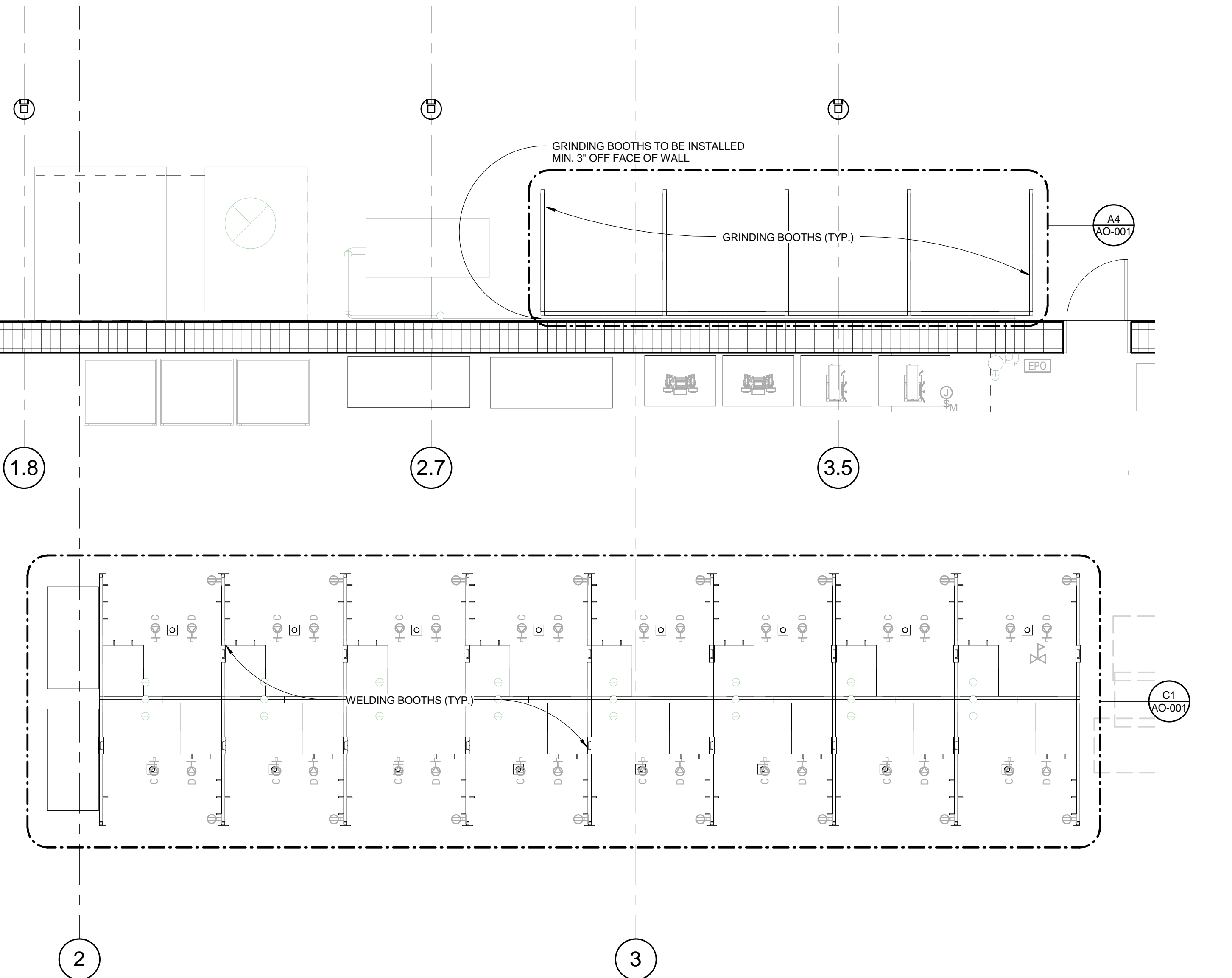
A1 ENLARGED PLAN - WELDING LAB 1/4" = 1'-0"
