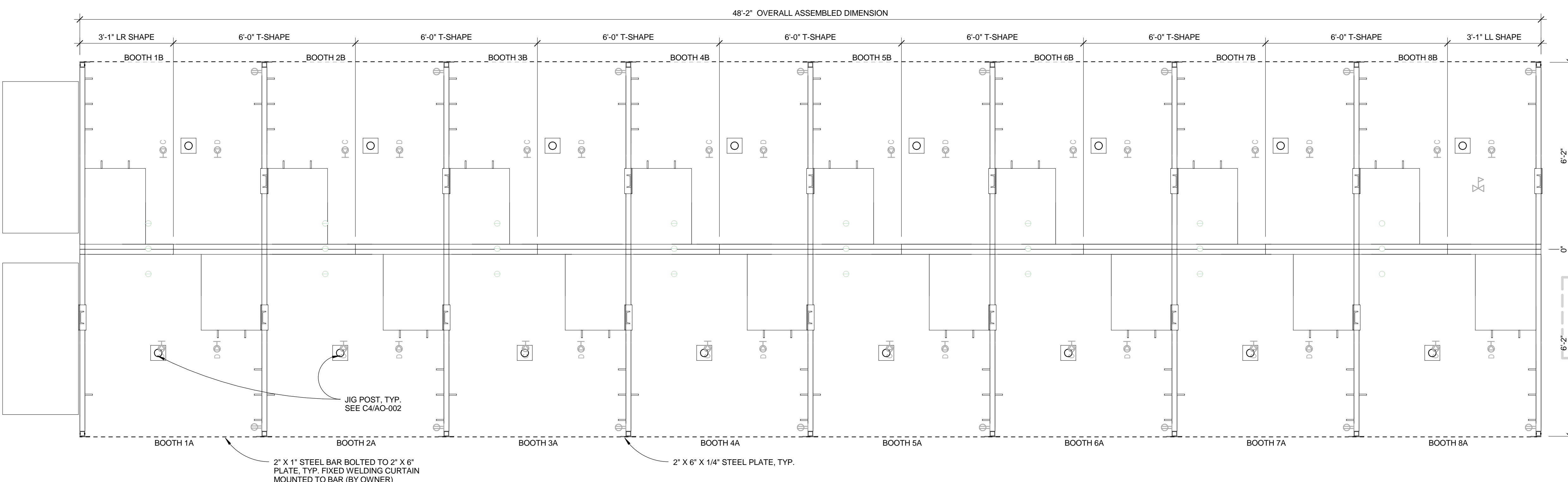
C1 ENLARGED PLAN - WELDING BOOTHS 1/2" = 1'-0"
