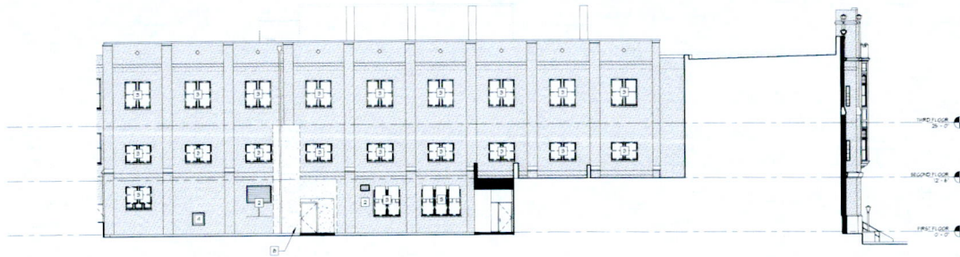
6 EXISTING WEST ELEVATION - GYM 3/12' x 7'4"
