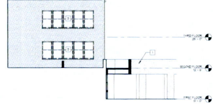
5 EXISTING EAST ELEVATION - BEYOND GYM 3/12' x 7'4"
